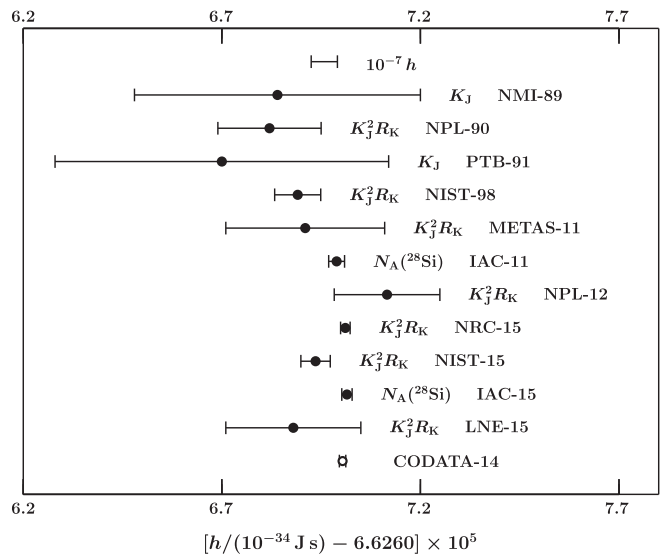
FIG. 3. Values of the Planck constant h with u_r < 10^{-6} inferred from the input data in Table XVIII and the 2014 CODATA recommended value in chronological order from top to bottom (see Table XXI).
